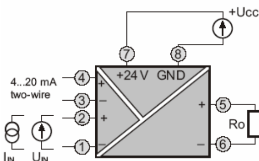
Electrical diagram
