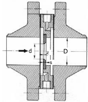
Execution with monolithic support
