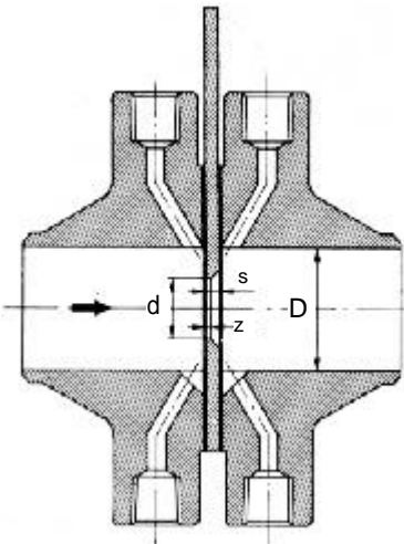
Execution corner taps type for 18" and larger.
