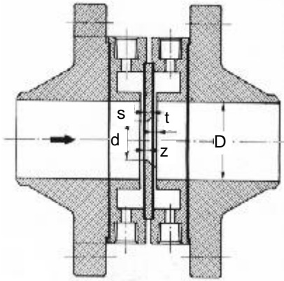
Execution with piezometric rings recommended up to 16" (DN 400) included
